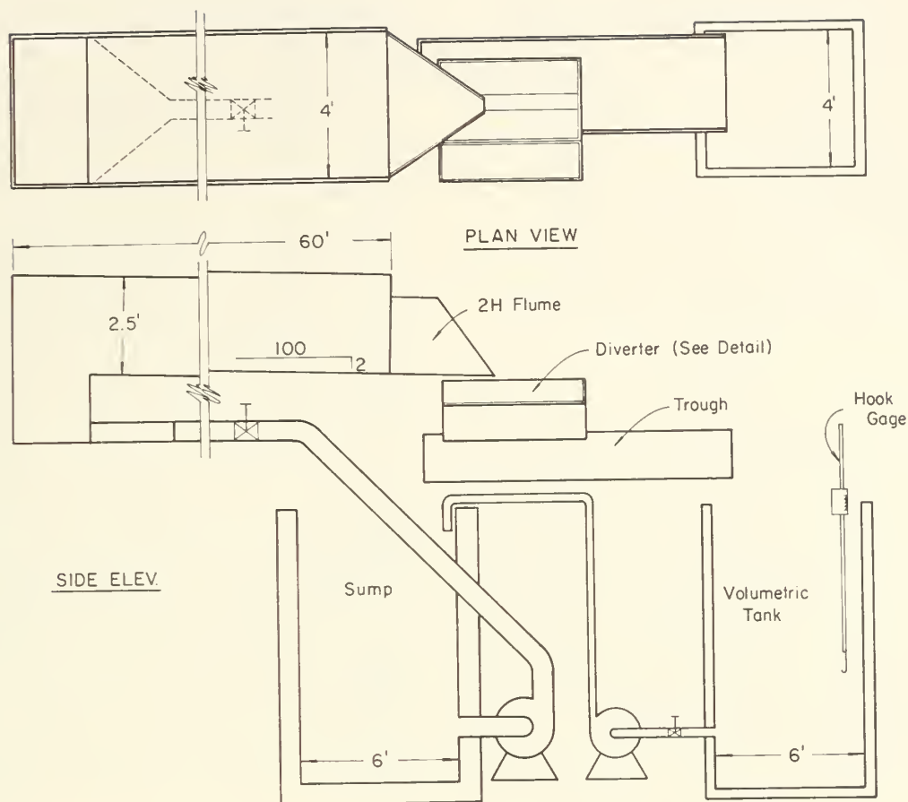
Figure 2.—Laboratory test apparatus.
